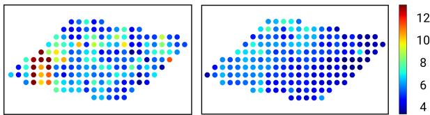
Figure 3: Error (cubic root metric) between the interpolated image, i_i , and the rendered one, \text{Render}(\pi_i) , for a set of uniformly distributed points along the manifold. We show the error when optical parameters \pi_i are computed through parameter interpolation (left), and by means of inverse rendering (right).
